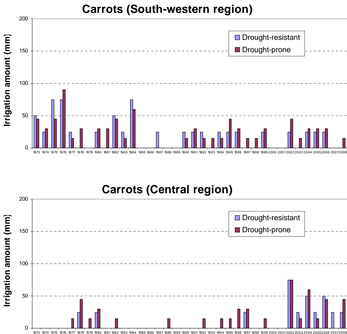
Figure 3.9. Irrigation requirement (mm) for late carrots in some other regions, 1973-2008.
