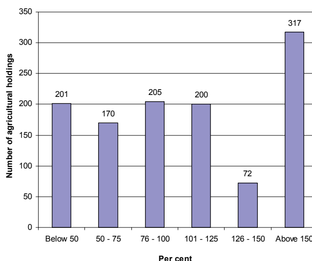
Figure 4.1. Number of agricultural holdings by proportion of potentially irrigated area (2007) in relation to crop areas (vegetables, potatoes and cereals) from applications for subsidies for 2007
