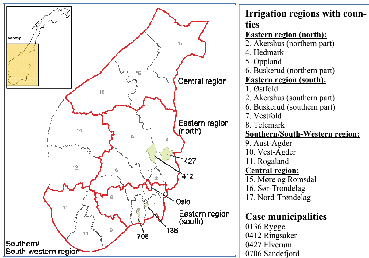
Figure 2.1. Distribution of counties in the irrigation regions included in this study
