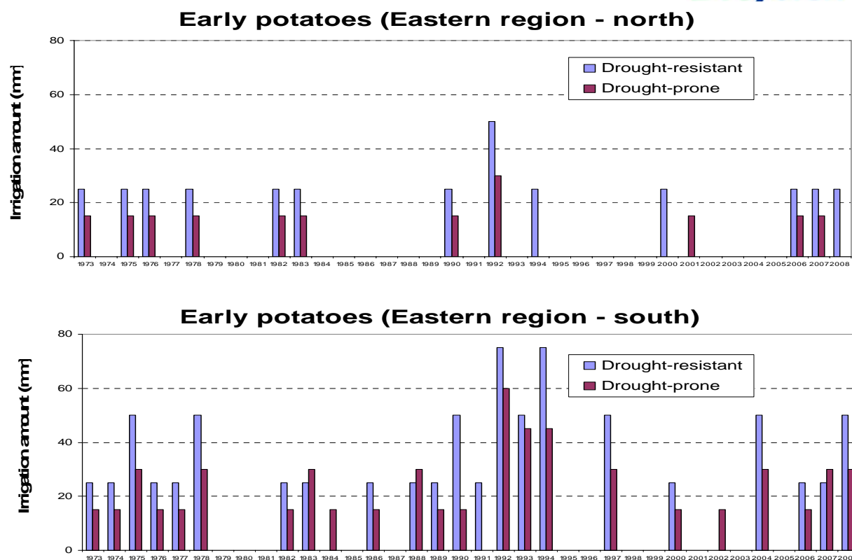
Figure 3.6. Irrigation requirement (mm) for early potatoes in Eastern Norway, 1973-2008.
