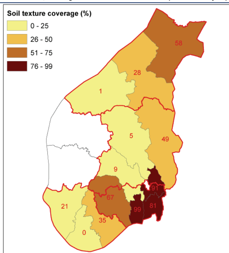
Figure 2.2. Soil texture, coverage for counties in the southern part of Norway in per cent
