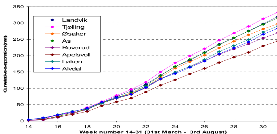
Figure 2.7. Cumulative evaporation values calculated for 2008 using the local equation for a number of Bioforsk's automatic weather stations in Eastern and Southern Norway.
