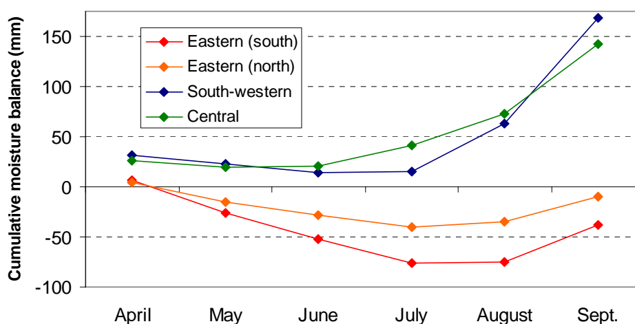
Figure 2.12. Cumulative water balance (sum of precipitation minus reference evaporation) in the four irrigation regions used in this study. Mean data for the period 1973-2008.
