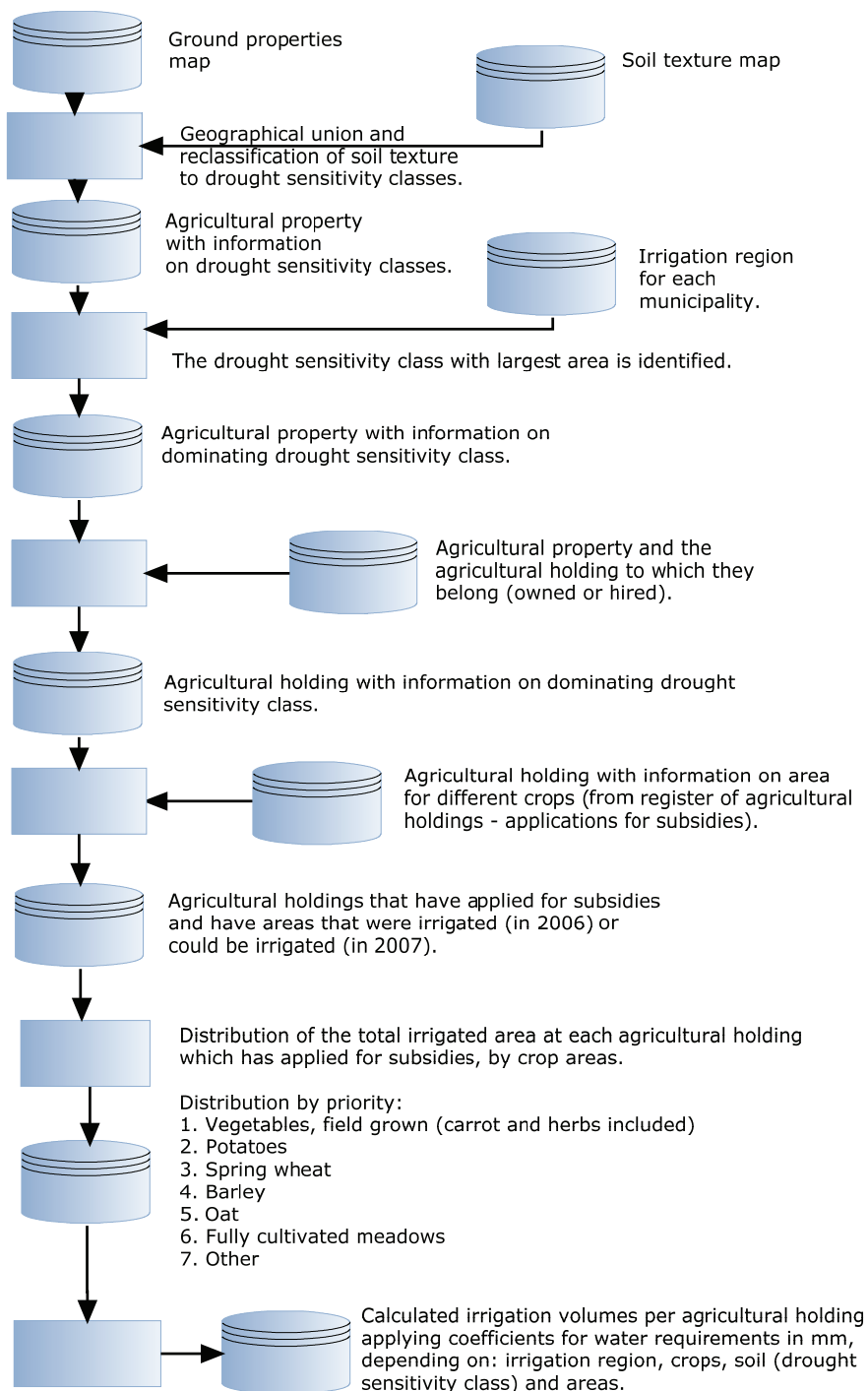
Figure 2.3. “Work flow” in development of model for calculation of irrigation volumes at -agricultural holding-level.
