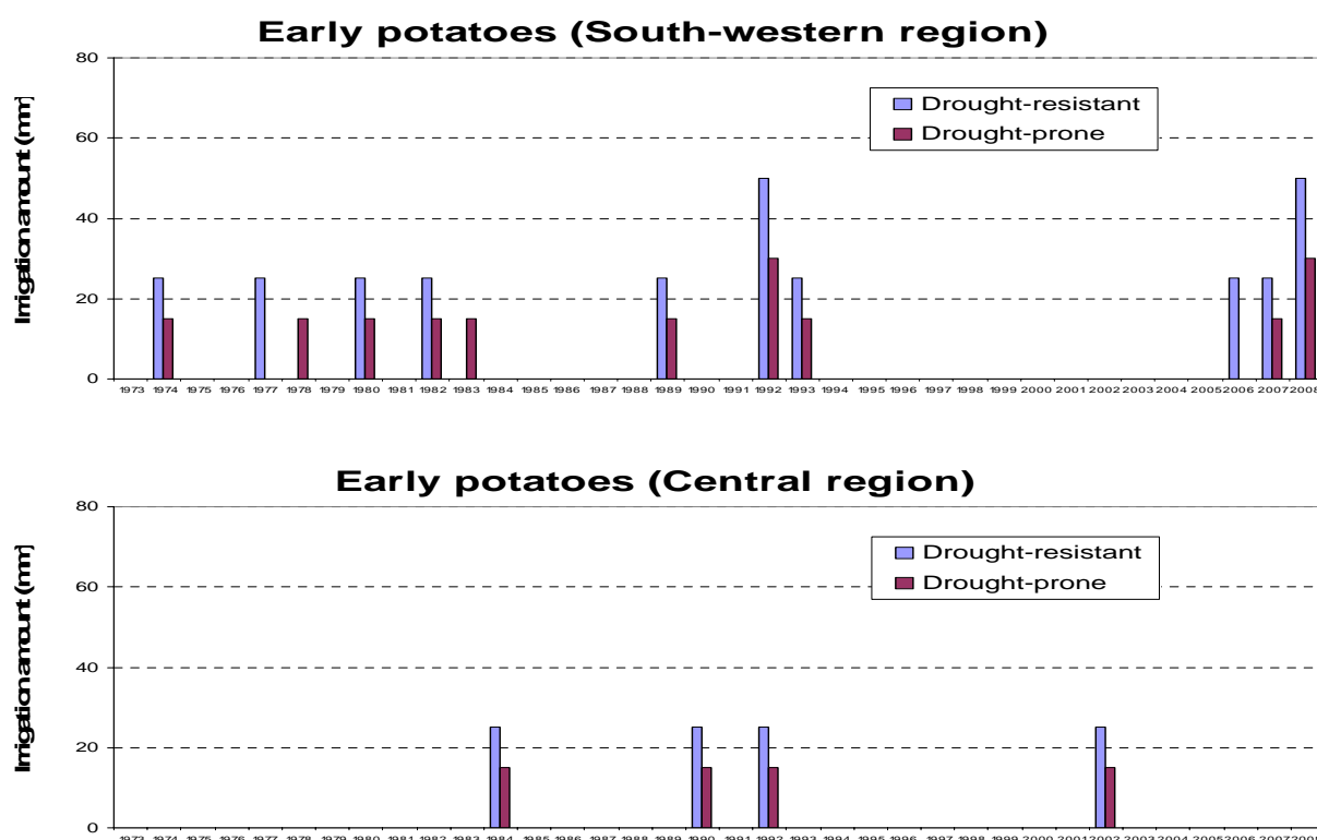
Figure 3.7. Irrigation requirement (mm) for early potatoes in some other regions, 1973-2008.
