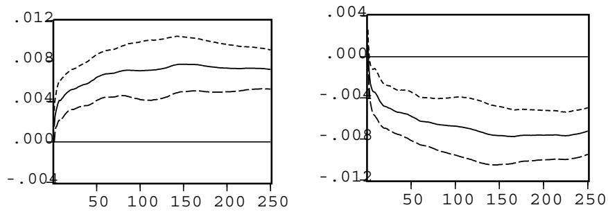
Figure 2: The coefficient for flows of (a) Financial and (b) Non-Financial customers, respectively, for different time horizons
