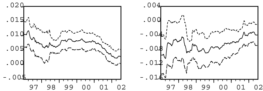
Figure 3: Rolling estimations of the coefficient ( \pm 2SE ) using a 3-year window
