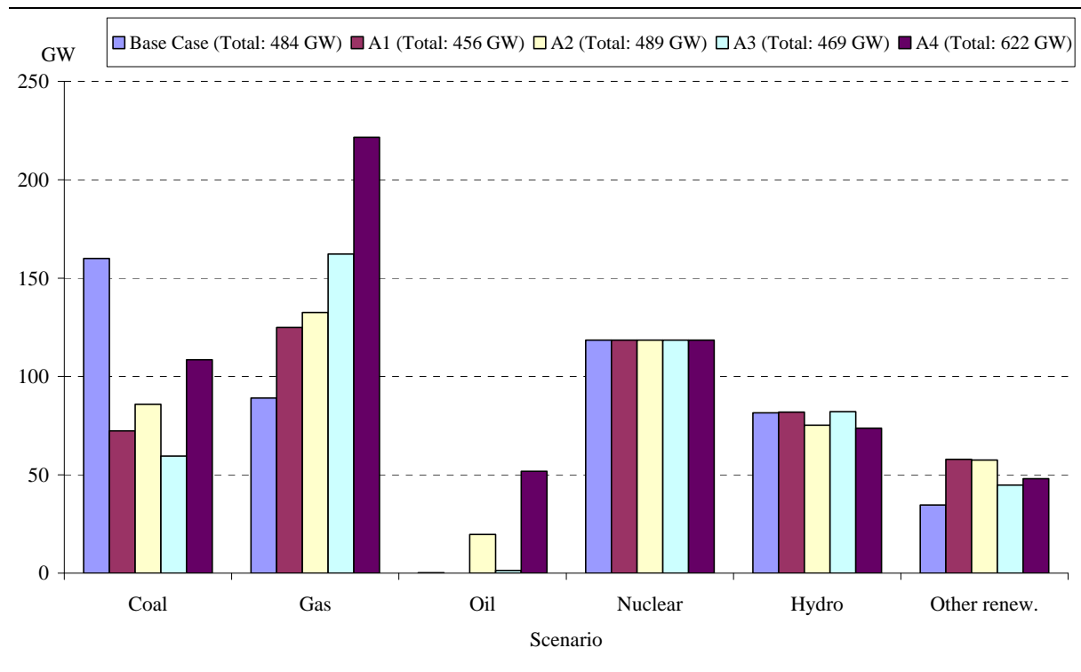
Figure A1. Maintained capacity of electricity by technologies under different allocation mechanisms. Policy scenario 2. GW
